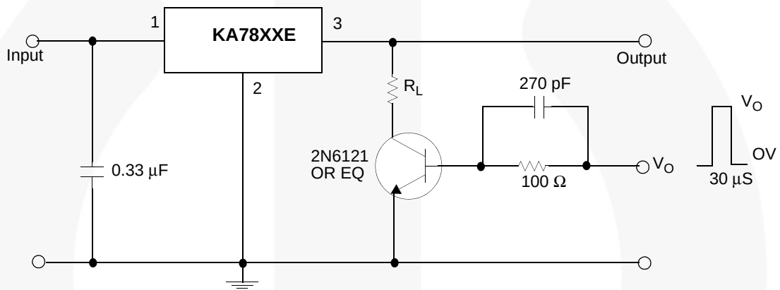
Figure 7. Load Regulation
